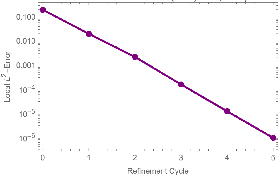
Local L^2 -Error at \alpha = (0.25, 0.25, 0.25)
